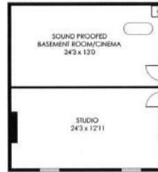
BASEMENT
