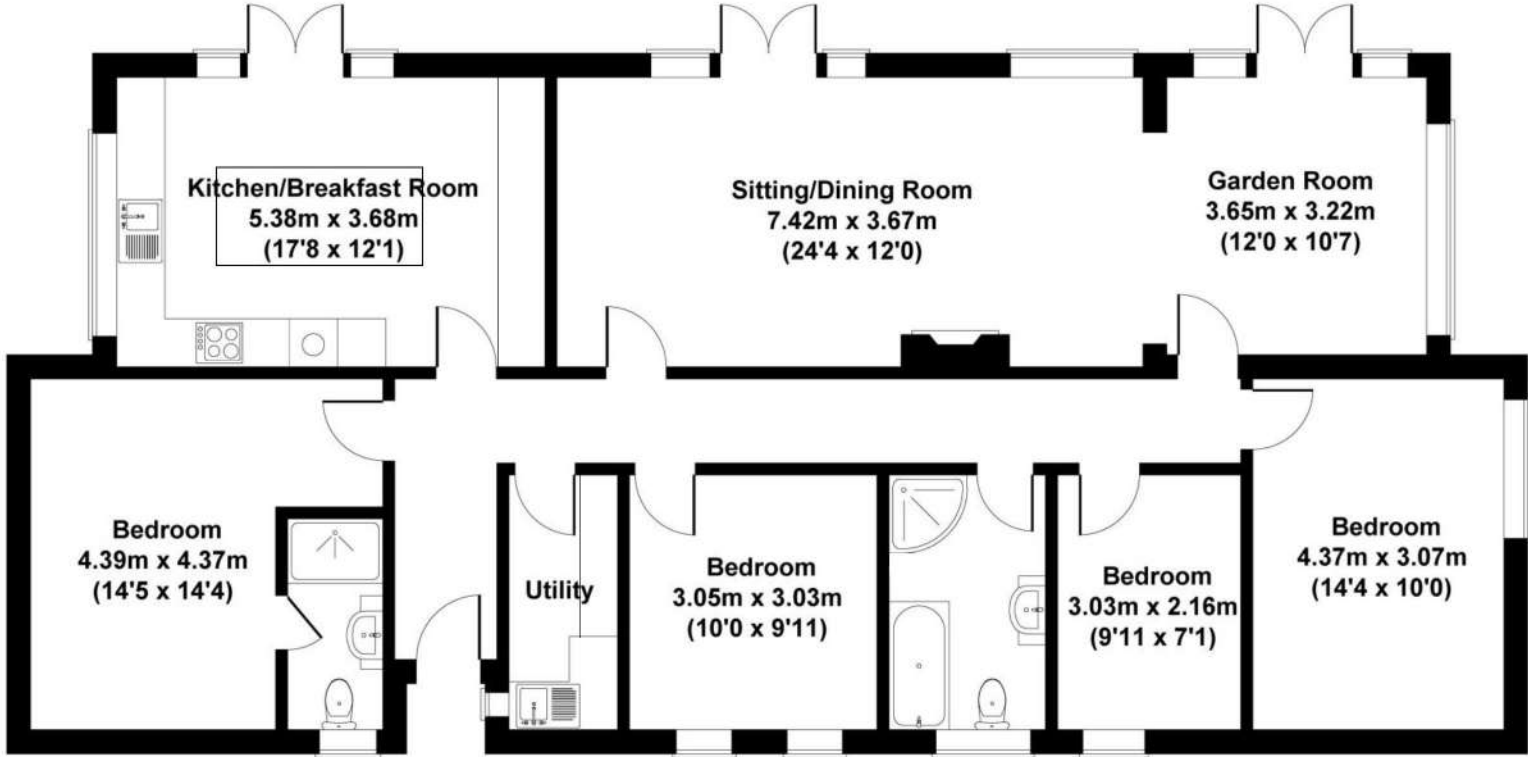
GROUND FLOOR
