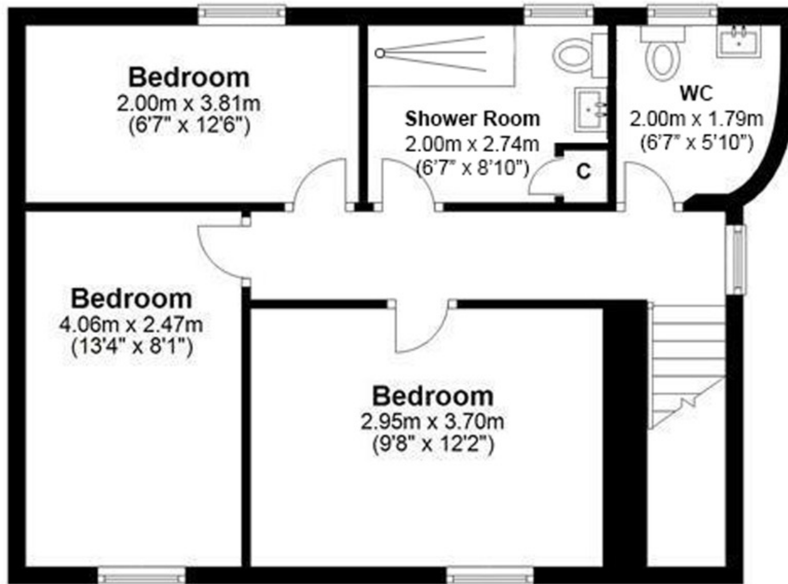
First Floor
