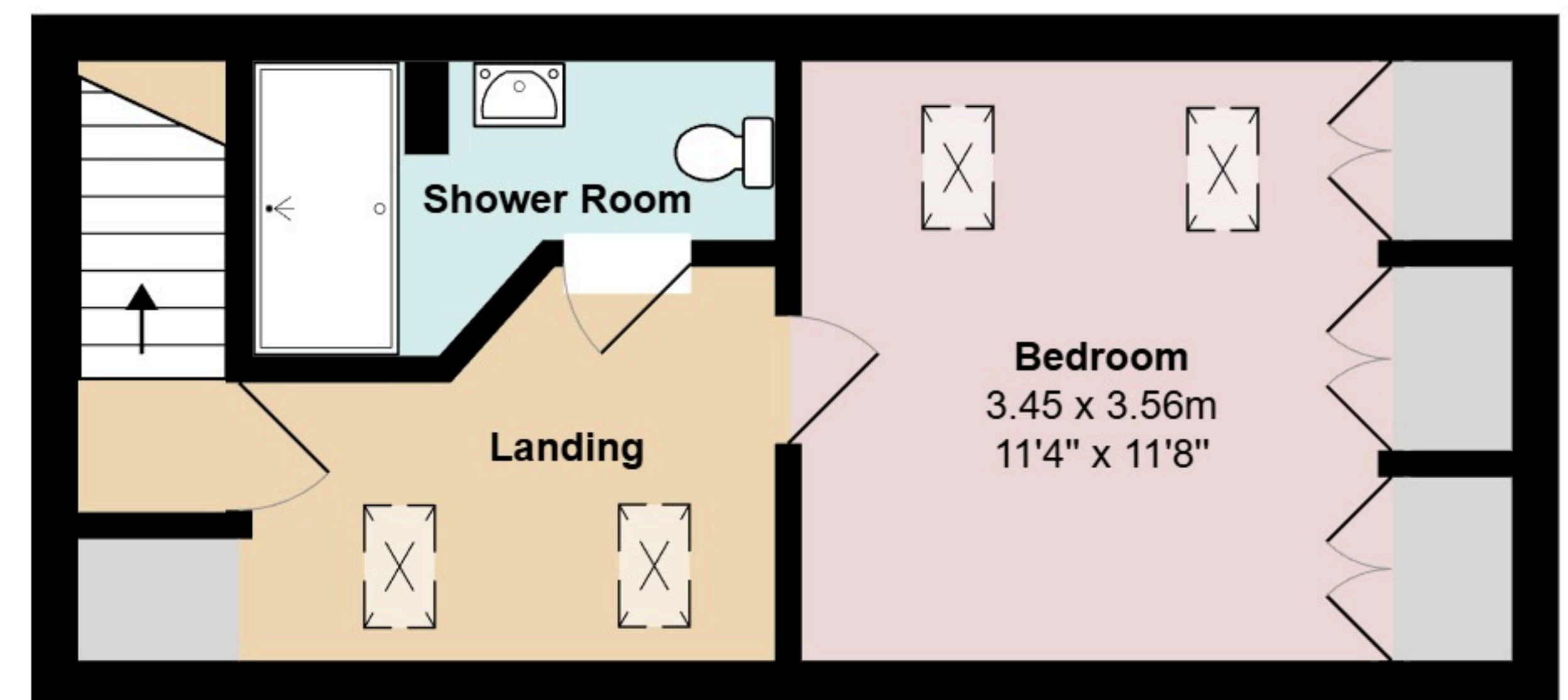
First Floor
