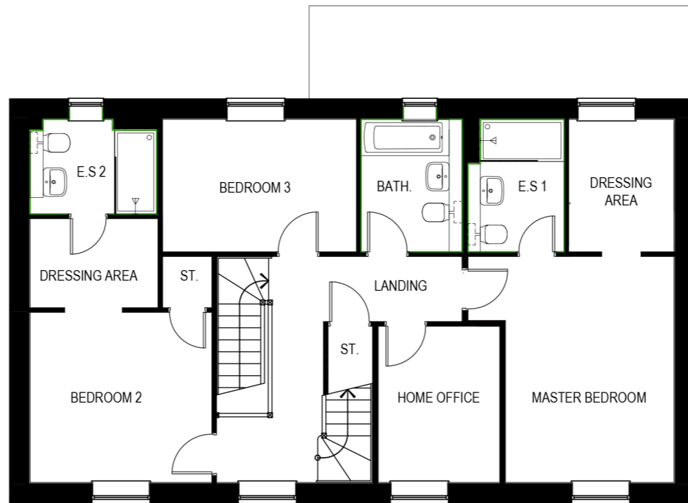
FIRST FLOOR
