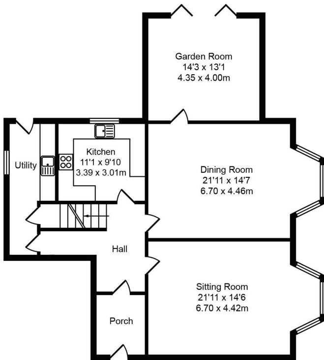
Ground Floor Approx. Floor Area 1160 Sq.Ft (107.8 Sq.M.)
