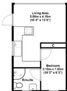
Annex Approx 28.00 Sq meters (301.00 Sq feet).
