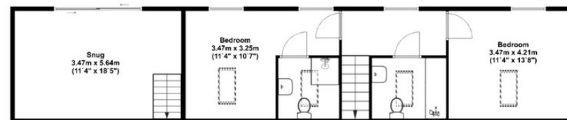
Second Floor Approx 65.00 Sq meters (700.00 Sq feet).
