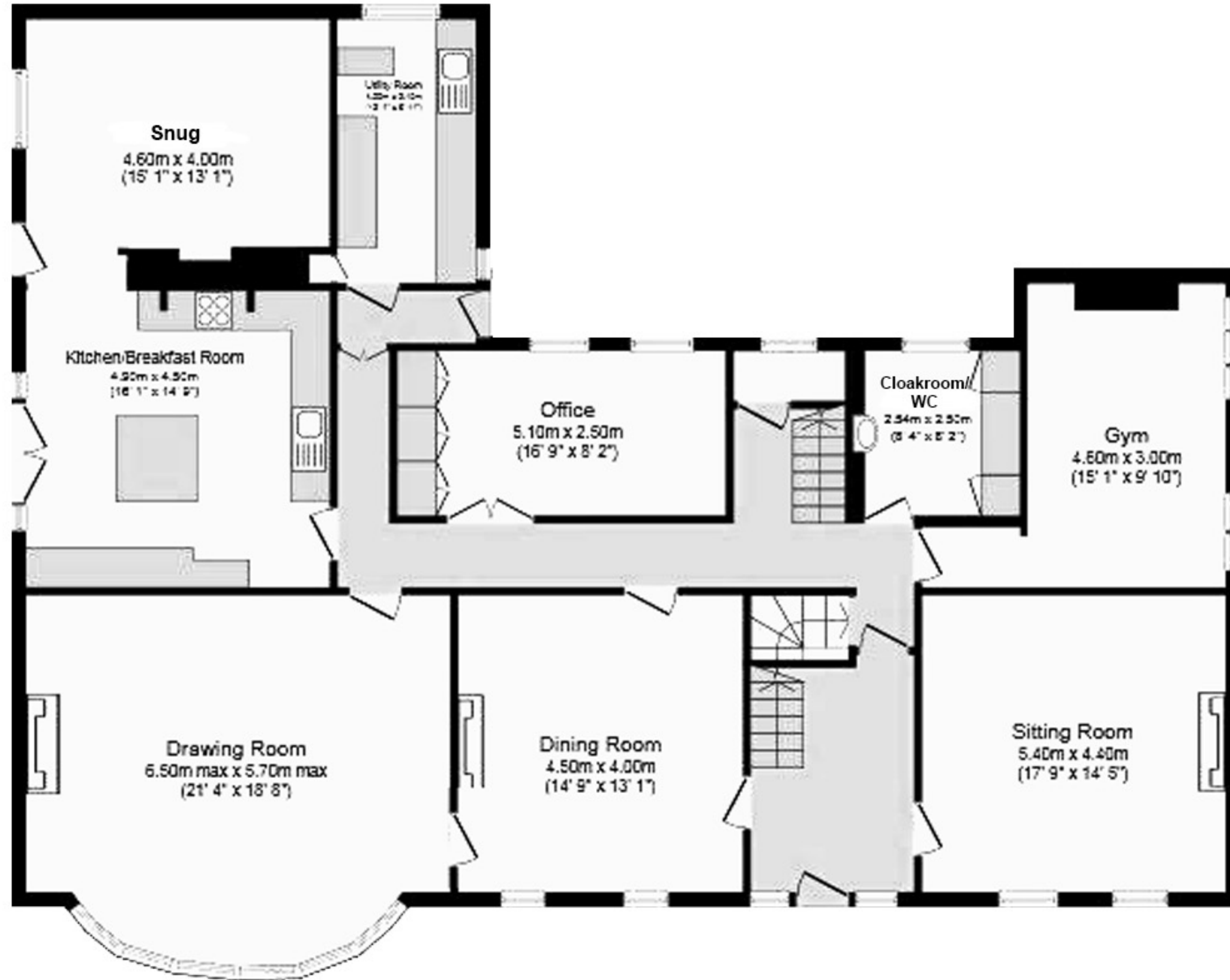
Ground Floor
