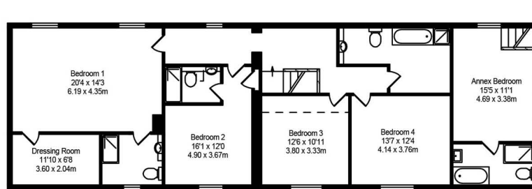
First Floor Approx. Floor Area 1511 Sq.Ft (140.38 Sq.M.)
