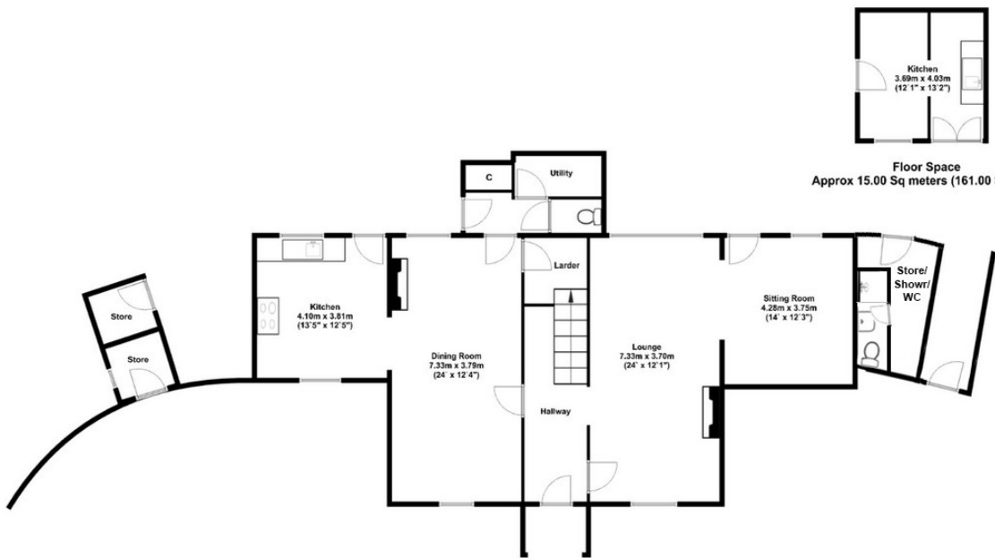
Ground Floor Approx 116.00 Sq meters (1249.00 Sq feet).
