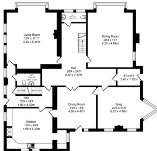
Ground Floor Approx. Floor Area 2126 Sq Ft (197.5 Sq.M.)
