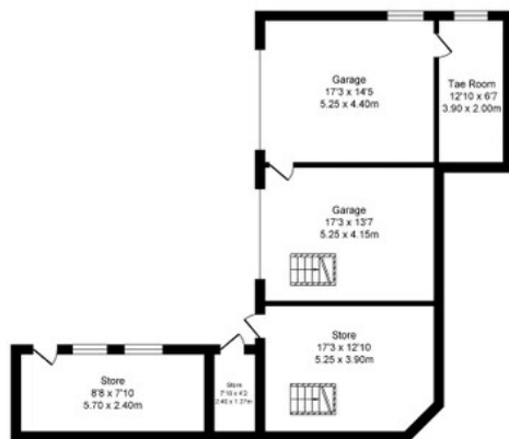
Garage Ground Floor Approx. Floor Area 1013 Sq Ft (94.1 Sq.M.)
