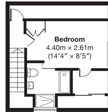
Annexe first floor area: 29.2 sq metre (315 sq feet)
